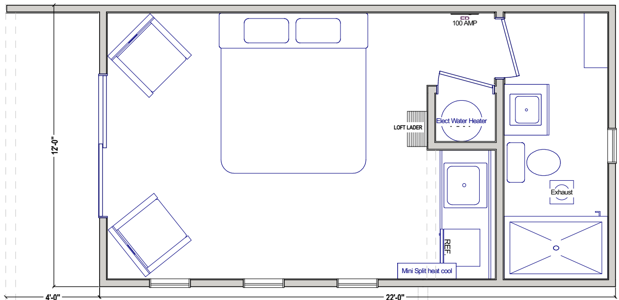
FLOOR PLAN 264 sq ft + loft
