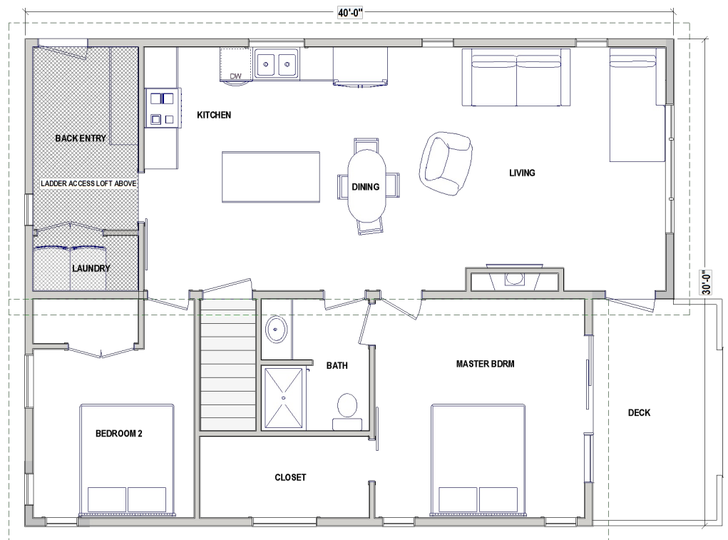
FLOOR PLAN 1130 sq ft
