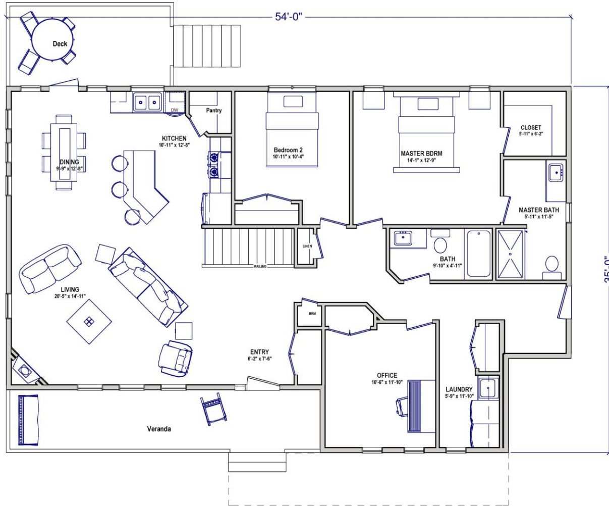
WYNDHAM FLOOR PLAN 1656 sq ft
