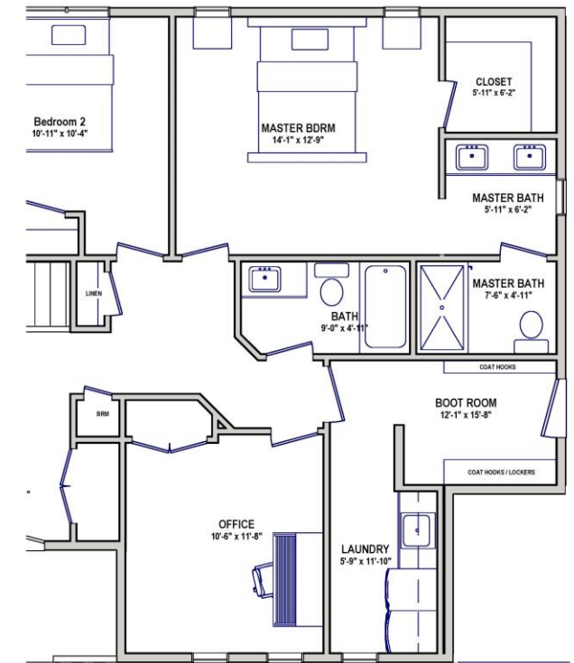
Alternate Master Bath / Boot Room / Laundry layout.
