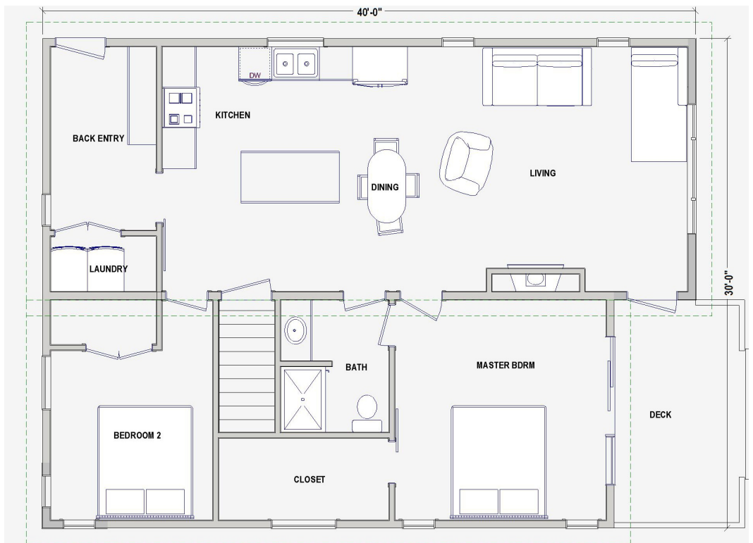
FLOOR PLAN 1130 sq ft
